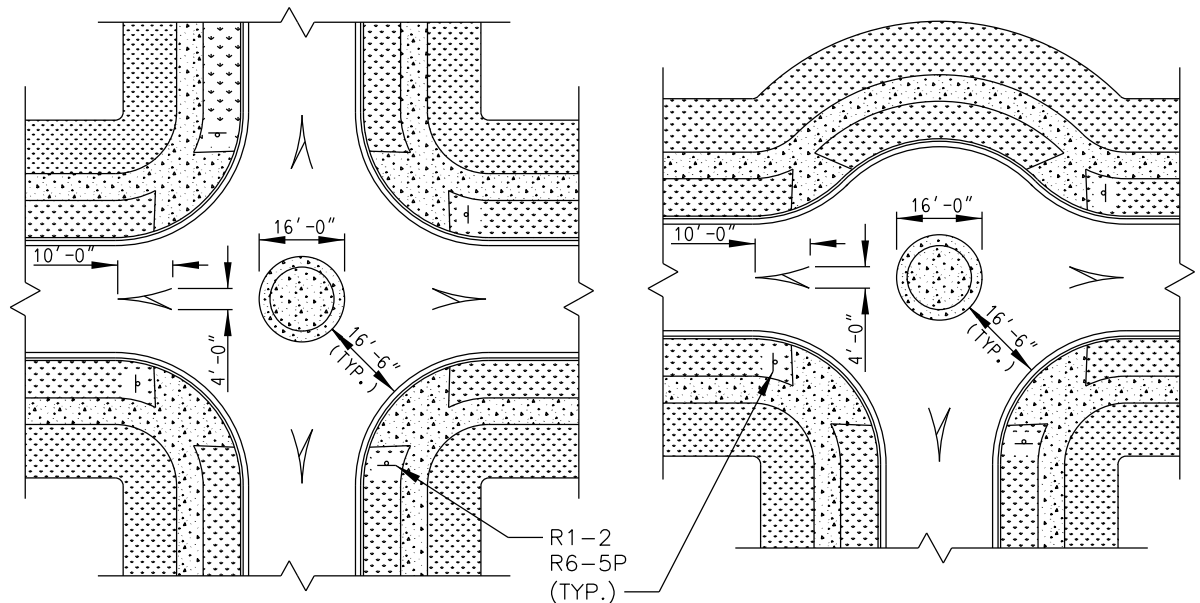
4-LEG PLAN VIEW
