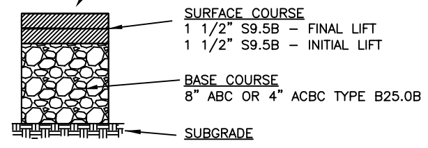
TYPICAL PAVEMENT SECTION
